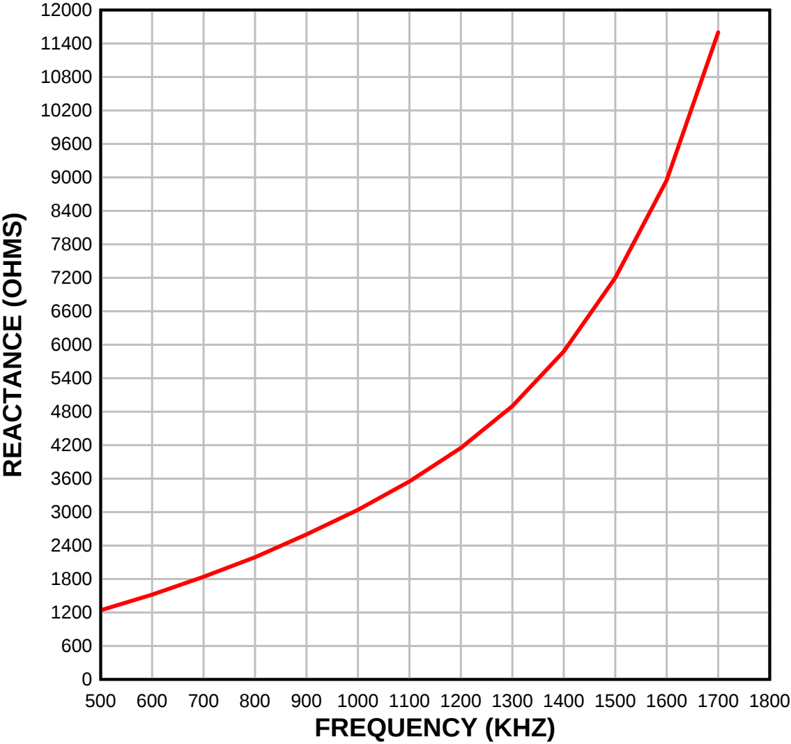
PHASETEK INC. MEASURED P600-160-2, 3 WIRE LIGHTING CHOKE
